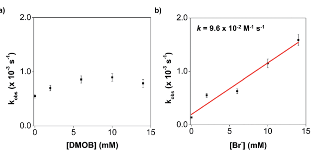
Fig. 5 Kinetic experiments performed to probe the mechanism for the formation of \mathbf{1}\text{-TAML}(\text{X}) . Plot of k_{\text{obs}} against the concentration of (a) DMOB and (b) \text{Br}^- . The linear fit of the data in (b) gives a second-order rate constant, k , for the aromatic substitution of oxidised \mathbf{1}(\text{Br}) .
