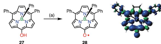
Fig. 10 Synthesis of the subporphyrin meso -oxy radical 28 (isovalue = 0.001). (a) 800 equiv. \text{PbO}_2 , \text{CH}_2\text{Cl}_2 , rt, quant.
