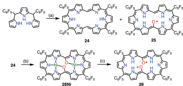
Fig. 9 Hexaphyrin mono- and bis( meso -oxy) radicals. (a) 22 equiv. \text{HC}(\text{OMe})_3 , 17 equiv. \text{MeSO}_3\text{H} , MS3A, \text{CH}_2\text{Cl}_2 , 0 °C, 7 h in the dark, 17% for 24 and 15% for 25 ; (b) ca. 10 equiv. \text{Ni}(\text{acac})_2 \cdot n\text{H}_2\text{O} , \text{CH}_2\text{Cl}_2/\text{MeOH} , rt, 1 h, 24%; (c) ca. 900 equiv. \text{MeSO}_3\text{H} , \text{CH}_2\text{Cl}_2 , rt, 30 min, 83%.
