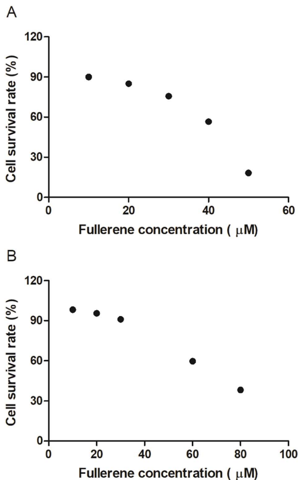
Fig. 6 Cytotoxic concentration of C_{62}(\text{COONa})_4 (A) and C_3 - C_{63}(\text{COONa})_6 (B) by \text{CC}_{50} .
