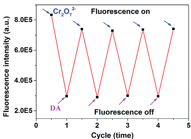
Fig. 6 Fluorescence intensity changes at 340 nm of PNCd/Cr(VI) upon alternate addition of concentrations of 160 \mu\text{M} Cr(vi) and 160 \mu\text{M} DA in PBS (pH: 7.4).
