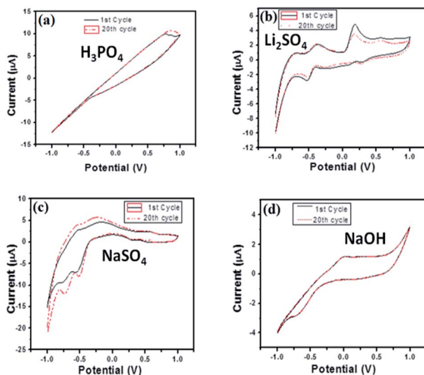
Fig. 13 Cyclic voltammograms of the \text{BiVO}_4/\text{FeVO}_4 modified GCE in mixed (a) 0.1 M \text{H}_3\text{PO}_4 , (b) 0.1 M \text{Li}_2\text{SO}_4 , (c) 0.1 M \text{NaSO}_4 , (d) 0.1 M \text{NaOH} and ascorbic acid (0.5 mM) solutions. Scan rate = 50 \text{ mV s}^{-1} . Recycling for 1 st and 20 th time.
