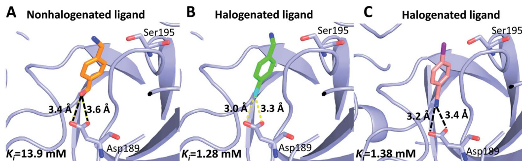
Fig. 5 Comparison of halogenated and nonhalogenated inhibitors to the protein target (uPA). uPA in complex with the nonhalogenated ligand 4-(aminomethyl-phenyl)-methanol ((A) PDB code 3KHV), its brominated analog 4-bromobenzylamine (B) and iodinated analog 4-iodobenzylamine (C). The polypeptides backbone are traced as a lightblue ribbon, with amino acids and ligands involved in halogen bonding interactions and hydrogen bonds (black dashed lines) shown as ball stick models with carbons (orange, green and pink, respectively), oxygen (red), nitrogen (blue), bromine (cyan), and iodine (purple).
