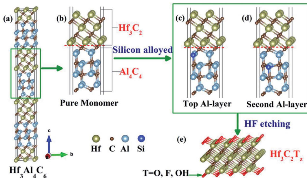
Fig. 2 Schematic illustration of the synthesis of \text{Hf}_3\text{C}_2\text{T}_z MXene from nanolaminated phase \text{Hf}_3[\text{Al}(\text{Si})]_4\text{C}_6 . (a) Structure of \text{Hf}_3[\text{Al}(\text{Si})]_4\text{C}_6 , (b) structure of pure \text{Hf}_3\text{Al}_4\text{C}_6 monomer, (c) and (d) structure of two \text{Hf}_3\text{Al}_4\text{C}_6 monomers with different silicon alloying, and (e) side view of \text{Hf}_3\text{C}_2\text{T}_z MXene. Reprinted with permission of ref. 36 Copyright 2017 American Chemical Society.
