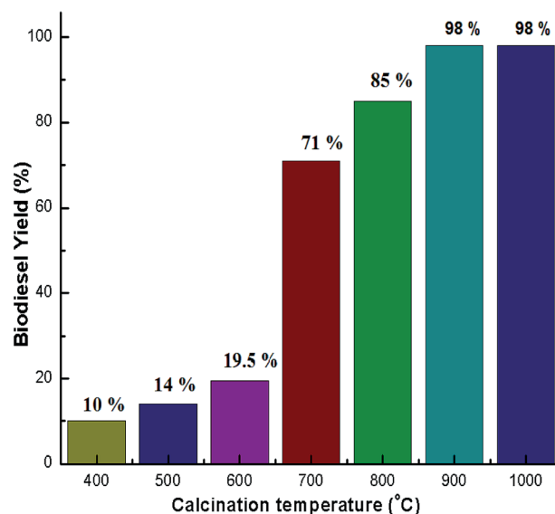
Fig. 7 Effect of calcination temperature on biodiesel yield obtained under optimised conditions: 6 : 1 methanol to oil ratio, 3.5 wt% catalyst loading, time 7 h and temperature of 28 °C (room temperature).
