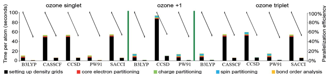
Fig. 20 Parallelization timing and efficiency results for ozone singlet, +1 doublet, and triplet at different levels of theory: B3LYP/6-311+G*, CASSCF/AUG-cc-pVTZ, CCSD/AUG-cc-pVTZ, PW91/6-311+G*, and SAC-CI/AUG-cc-pVTZ. Serial and 16 parallel processors calculations are compared.
