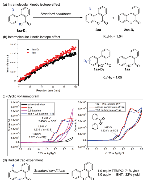
Scheme 6 Mechanism studies.
