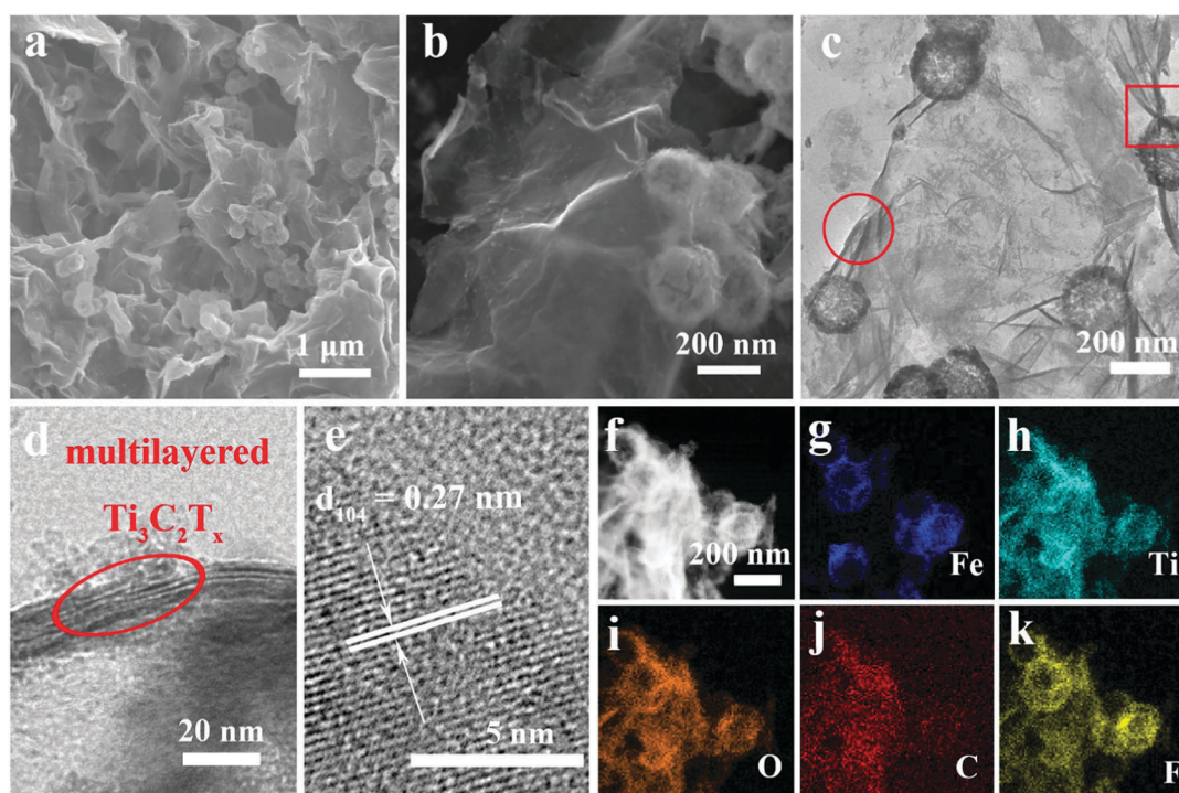
Fig. 2 (a and b) SEM images of the aerogel-like \text{Ti}_3\text{C}_2\text{T}_x@ \text{Fe}_2\text{O}_3 composite. (c) TEM image of the aerogel-like \text{Ti}_3\text{C}_2\text{T}_x@ \text{Fe}_2\text{O}_3 composite. (d and e) HRTEM images of the \text{Ti}_3\text{C}_2\text{T}_x@ \text{Fe}_2\text{O}_3 composite. The circle and box in panel (c) correspond to the HRTEM images for the selected area of panel (d) and (e), respectively. (f–k) Elemental mapping of the \text{Ti}_3\text{C}_2\text{T}_x@ \text{Fe}_2\text{O}_3 composite.
