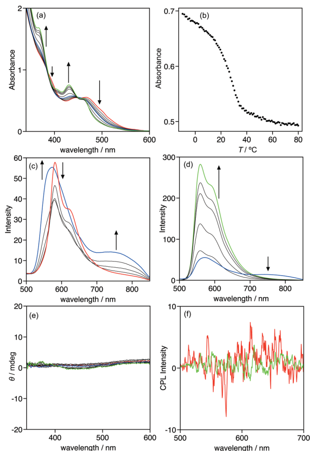
Fig. 4 (a) Temperature-dependent UV-vis absorption spectra of 1 in MCH. The spectra were recorded every 10 °C. The arrows indicate the change in the spectra as the temperature decreases from 80 to -10 °C. (b) Plot of the absorbance at 430 nm of 1 in MCH. (c and d) Temperature-dependent emission spectra of 1 in MCH. The spectra were recorded every 10 °C. The arrows indicate the change in the spectra as the temperature decreases from (c) 80 to 40 and (d) 40 to -10 °C. (e) Temperature-dependent CD spectra of 1 in MCH. The spectra were recorded every 10 °C from 80 to -10 °C. (f) Temperature-dependent CPL spectra of 1 in MCH at 80 and -10 °C. Red, blue, and green lines display the spectra at 80, 40, and -10 °C, respectively. [\mathbf{1}] = 1.5 \times 10^{-4} \text{ mol L}^{-1} ; \lambda_{\text{ex}} = 430 \text{ nm} ; l = 0.1 \text{ cm} .
