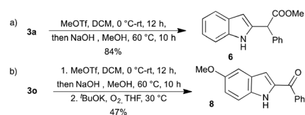
Scheme 5 Synthetic applications of the developed method.
