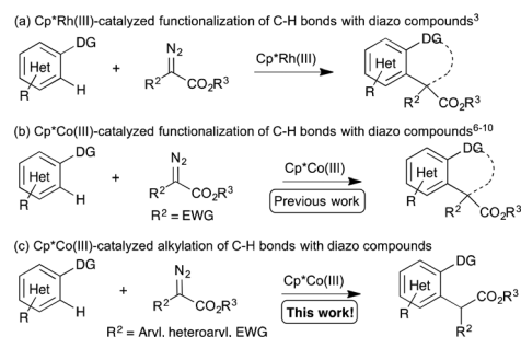
Scheme 1 Transition metal catalysed diazocoupling reactions.
