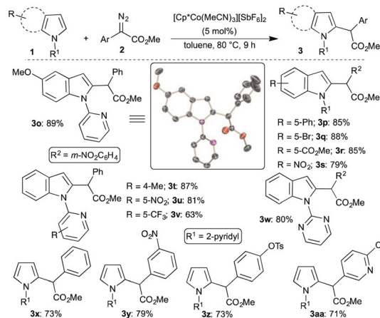
Scheme 3 Co-Catalysed selective C2-alkylation. Scope of indole derivatives.
