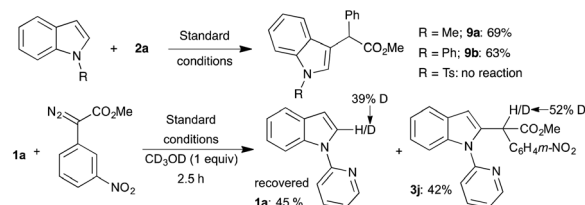
Scheme 6 Preliminary mechanistic investigation.
