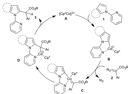
Scheme 7 Plausible mechanism.
