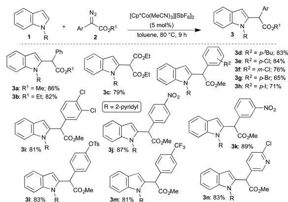
Scheme 2 Cobalt catalysed selective C2-alkylation. Scope of diazo compounds.
