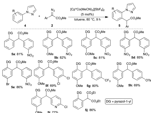
Scheme 4 Co-Catalysed selective alkylation of arenes.
