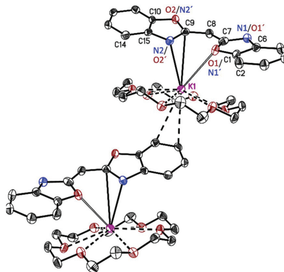
Fig. 3 Polymeric structure of [[\{(\text{NCOC}_6\text{H}_4)_2\text{CH}\}\text{K}(\text{18-crown-6})]_n ( 3 ). Anisotropic displacement parameters are depicted at the 50% probability level. Hydrogen atoms are omitted for clarity. Structural data are given in Table 1 and the Experimental.
