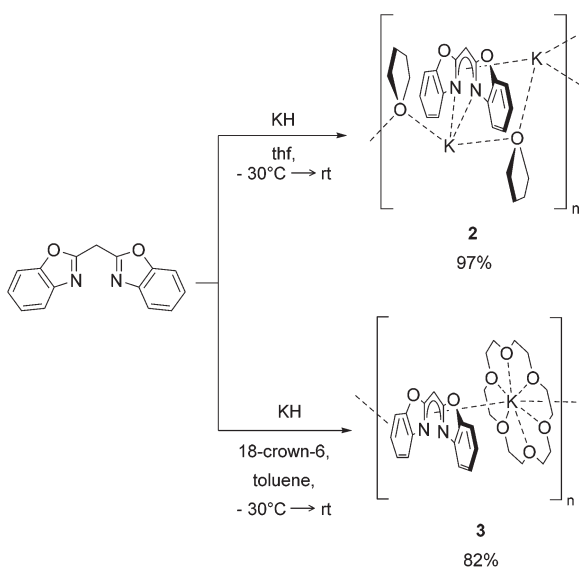
Scheme 2 Syntheses of [[\{(\text{NCOC}_6\text{H}_4)_2\text{CH}\}\text{K}(\text{thf})]_n ( 2 ) and [[\{(\text{NCOC}_6\text{H}_4)_2\text{CH}\}\text{K}(\text{18-crown-6})]_n ( 3 ) by deprotonation with KH.
