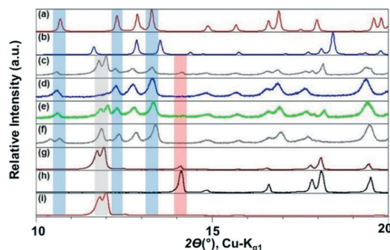
Fig. 1 Simulated pattern of the cocrystal, CAF–CA, Form I (P1) (a) and CAF–CA, Form II (P21/c) (b); the ground powder as obtained from [C 2 mim][NTf 2 ] (c), [C 2 mim][BF 4 ] (d), [OHC 2 mim][NTf 2 ] (e), [OHC 2 mim][BF 4 ] (f); experimental pattern of the powder mixture of CAF and CA obtained from neat grinding (g), and CA (h) and CAF (i) used in the grinding experiments.
