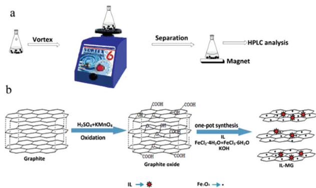
Fig. 1 Procedure of MDSPE (a), and one-pot synthesis of IL-MG (b).
