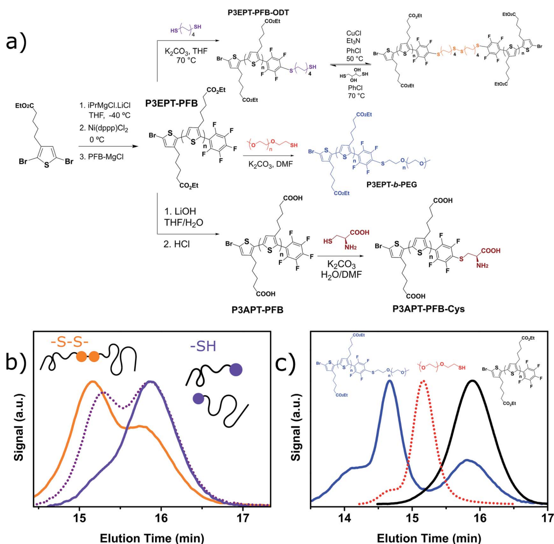
Fig. 5 (a) Synthesis of P3EPT-PFB and P3APT-PFB with model "click" reactions performed post-polymerization. (b) Gel permeation chromatography elugram ( 80^\circ C in chlorobenzene) of P3EPT-PFB-ODT in the thiol (purple) and disulfide (orange) forms. The dotted purple line illustrates partial reduction of the disulfide link (c) gel permeation chromatography elugram ( 80^\circ C in chlorobenzene) of P3EPT-PFB (black), mPEG-SH (red), and P3EPT- b -PEG (blue). Traces for all elugrams are obtained from a 450 nm diode array detector, except mPEG-SH which was measured using a refractive index detector.
