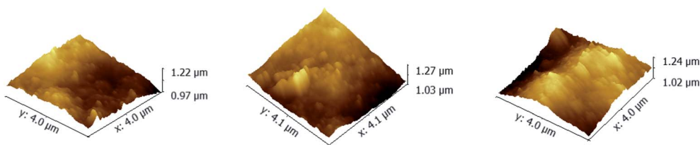
Fig. 4 AFM images of PAN-[PAH/(PSS-TPPS)] 6 membranes prepared from PAH solutions at pH 6.5 and PSS-TPPS solutions at pH values of 2.0 (A), 4.5 (B), and 8.0 (C).
