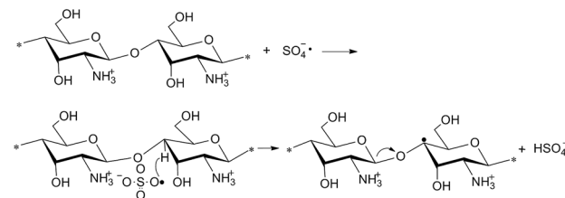
(2) Persulfate ion was attracted to the cationic amino group and free radical was transferred to the C-4 carbon
