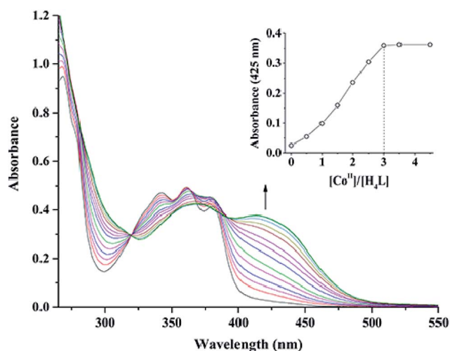
Fig. 1 UV-vis spectral changes of H_4L by the addition of Co(OAc)_2 ( CHCl_3/CH_3OH 3 : 2 v/v, [H_4L] = 2.5 \times 10^{-5}\text{ M} ). The inset shows the plot of absorbance at 425 nm versus the molar ratio [Co^{II}]/[H_4L] .
