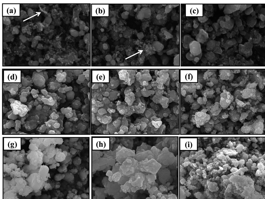
Fig. 8 SEM images of regenerated materials with doping new \text{LiFePO}_4 at different temperature and ratio: (a–c) 600^\circ\text{C} with doping at 1 : 9 to 3 : 7; (d–f) 700^\circ\text{C} with doping at 1 : 9 to 3 : 7; (g–i) 800^\circ\text{C} with doping at 1 : 9 to 3 : 7.
