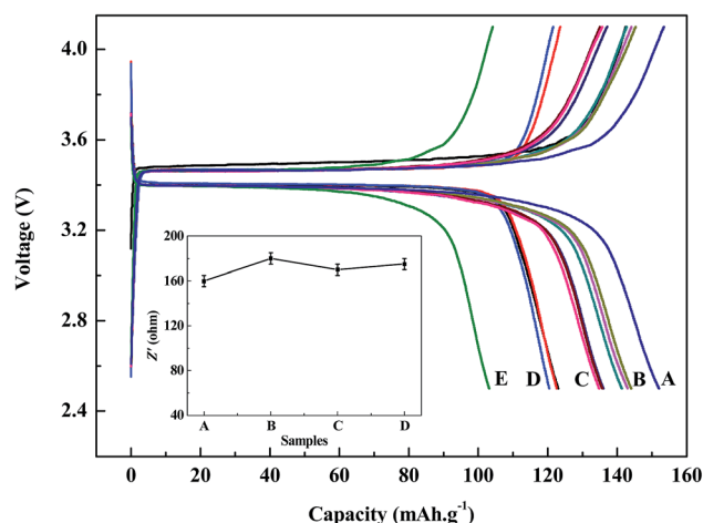
Fig. 9 Discharge/charge voltage and impedance profiles of regenerated \text{LiFePO}_4 at a current density of 0.1\text{C} : (A) commercial \text{LiFePO}_4 ; (B) 700^\circ\text{C} with the ratio of 1 : 9, 2 : 8, 3 : 7; (C) 600^\circ\text{C} with the ratio of 1 : 9, 2 : 8, 3 : 7; (D) 800^\circ\text{C} with the ratio of 1 : 9, 2 : 8, 3 : 7; (E) regenerated without doping new \text{LiFePO}_4 .
