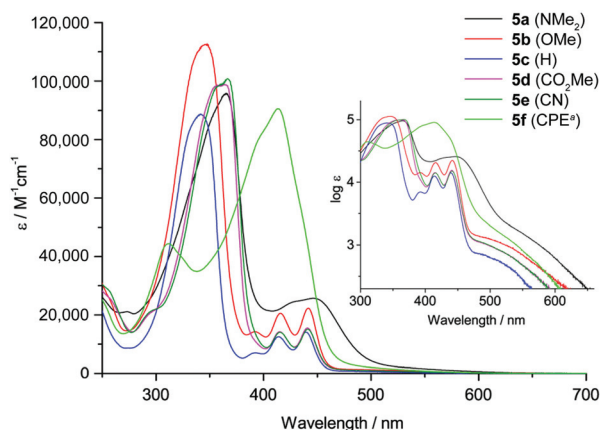
Fig. 2 Absorption spectra of 5a–f in CH 2 Cl 2 solution ( a CPE = CHC(CN)(CO 2 Et)). Inset: Spectra plotted on a logarithmic scale.
