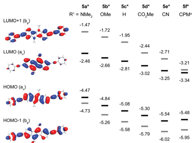
Fig. 1 Molecular orbitals of 5c* (R 1 = H, left) and energy diagram (eV, right) of calculated MOs of DBP derivatives 5a*–f* (TPSSH-D3/def2-TZVP, a CPM = CHC(CN)(CO 2 Me)).
