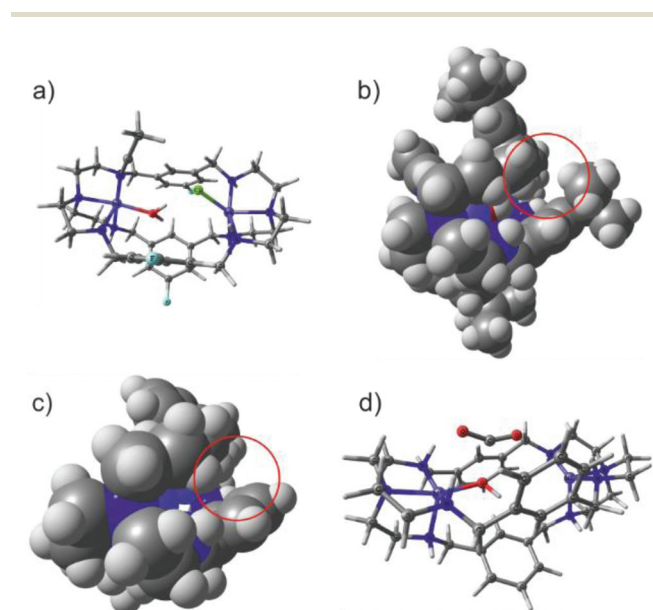
Fig. 5 (a) Geometry optimized structure of [Ni_2L_A^F] with Cl − , H 2 O and MeCN; (b) side view of [Ni_2L_A^{tBu}] , showing the steric hindrance of t Bu with the neighboring phenyl group; (c) side view of [Ni_2L_A^H] where steric effects are absent; (d) intermediate structure with bent CO 2 where CO 2 has been introduced near Ni 2+ at 2.2 Å, leading to barrierless C–O bond formation towards HCO 3 − .
