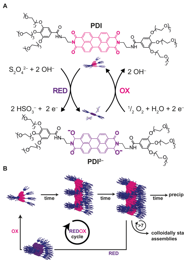
Fig. 12 Chemical fuels. (A) PDI was reduced upon addition of dithionite to the dianion PDI 2- , upon exposure to air PDI 2- is oxidized back to the neutral PDI. (B) The number and frequency of redox cycles will affect the outcome of the assemblies due to progressive changes in the assemblies after each redox cycle. Adapted from ref. 49 with permission from The Royal Society of Chemistry.
