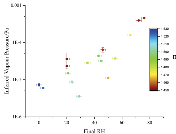
Fig. 9 Effective pure component vapour pressure estimates, determined for sucrose:malonic acid particles (prepared with a 5:1 mass ratio) via eqn (13) and (14) (closed circles). Points are coloured by the mean refractive index recorded after the initial water loss had ceased.
