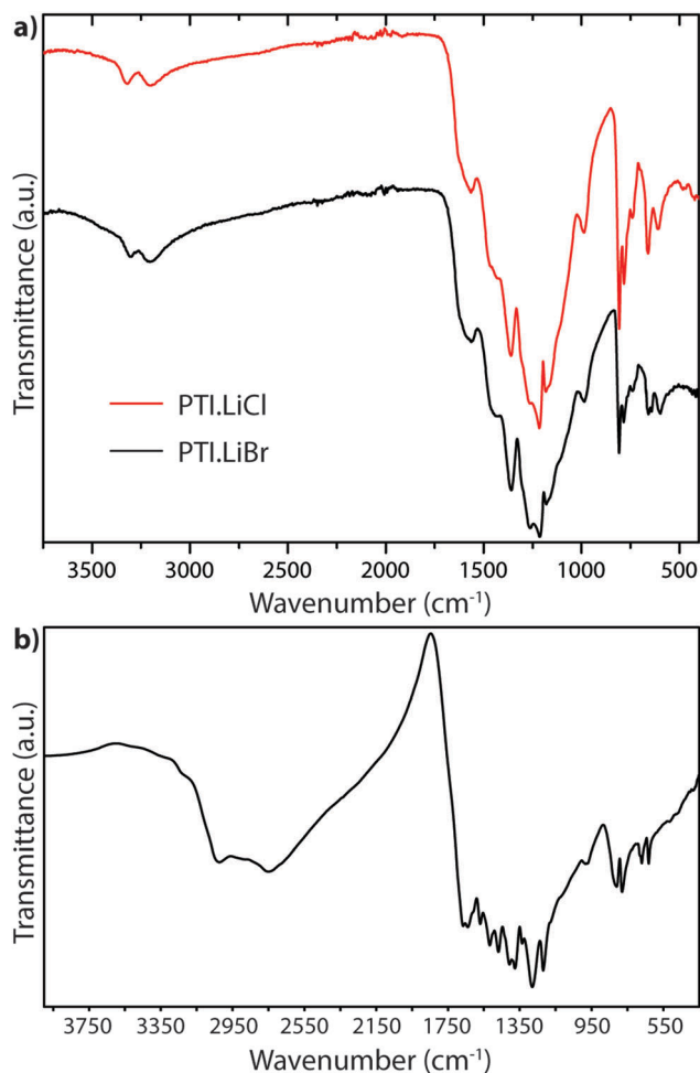
Fig. 18 FTIR powder transmission spectra for (a) PTI·LiCl and PTI·LiBr (b) PTI·HCl. 64
