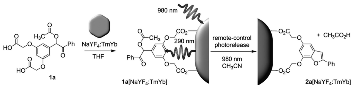
Fig. 5 UCNP-assisted photolysis at surfaces of UCNPs. Decoration of UCNPs with 3',5'-di(carboxymethoxy)benzoic cage 1a produces the remote-control release system ( 1a [NaYF 4 :TmYb]), which can be triggered by indirect irradiation with NIR light to generate 2a [NaYF 4 :TmYb] and release a carboxylic acid. Reproduced with permission. 71 Copyright 2010, Wiley-VCH Verlag GmbH & Co. KGaA.
