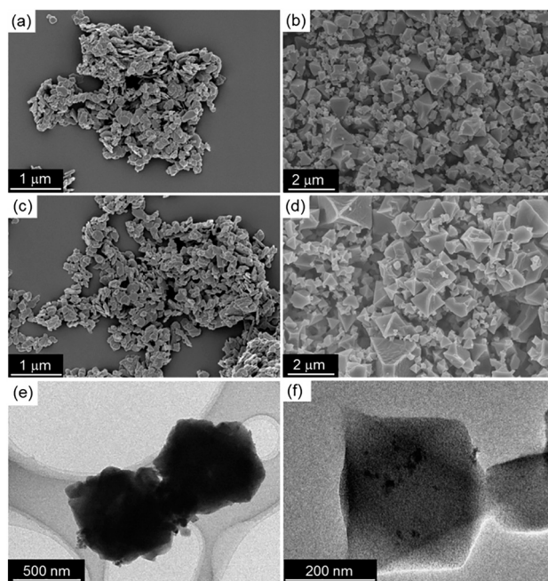
Fig. 2 SEM images of (a) \text{Fe}_3\text{O}_4@\text{Cu}_2(\text{OH})_3\text{NO}_3 , (b) \text{Fe}_3\text{O}_4@\text{HKUST-1} , (c) \text{Cu}_2(\text{OH})_3\text{NO}_3 and (d) HKUST-1. (e and f) TEM images of \text{Fe}_3\text{O}_4@\text{HKUST-1} .
