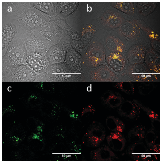
Fig. 5 Confocal fluorescence imaging of [TNPH] + in PC3 cells (37 °C, 15 minutes incubation, 10 mM 1:99 in cell media, \lambda_{\text{ex}} = 488 nm). Cells were pre-incubated with lysosome red tracker (1 \mu\text{M} 1:99 in cell media, 30 minutes incubation at 37 °C). (a) DIC channel; (b) overlay of the blue-green-red channels; (c) green channel ( \lambda_{\text{em}} = 500\text{--}550 nm); (d) red channel ( \lambda_{\text{em}} = 570\text{--}750 nm). Scale bar: 50 \mu\text{m} .
