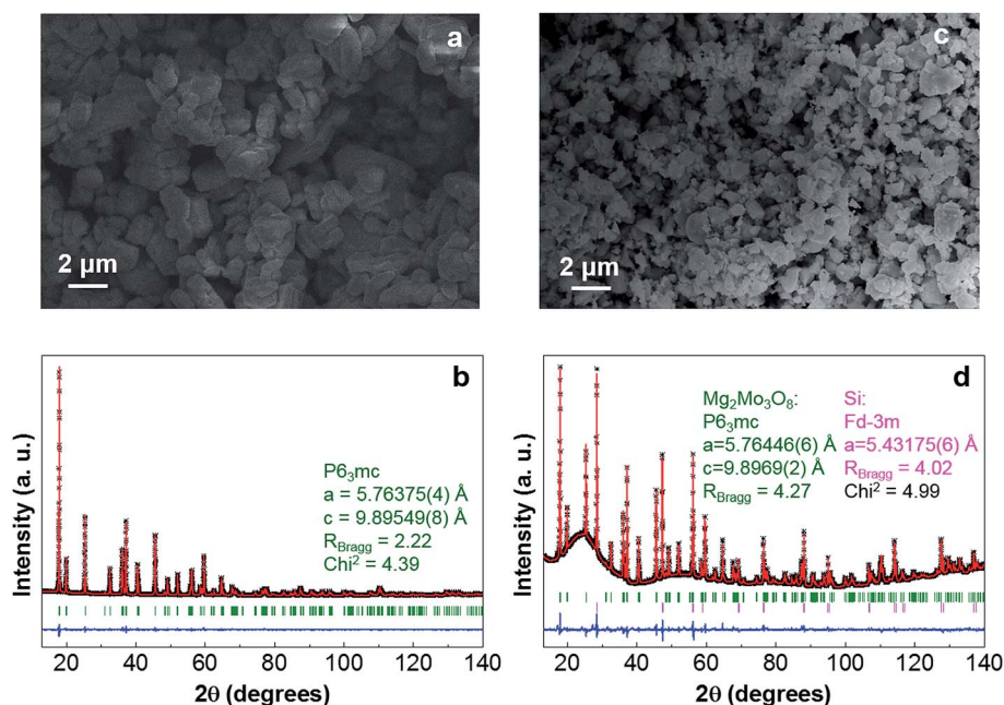
Fig. 2 (a) SEM image and (b) the Rietveld refinement fit of pristine \text{Mg}_2\text{Mo}_3\text{O}_8 (Bragg–Brentano geometry). (c) SEM image of the demagnesian sample. (d) Rietveld refinement of the demagnesian sample with the external silicon standard added to evaluate the percentage of the amorphous phase. The mixture was sealed in an X-ray capillary under Ar and was measured in a Debye–Scherrer geometry. Black crosses – experimental data, red lines – fitted data, blue line – difference map between observed and calculated data, green ticks – the P6_3mc phase of \text{Mg}_2\text{Mo}_3\text{O}_8 , pink ticks – the Fd\bar{3}m phase of Si.
