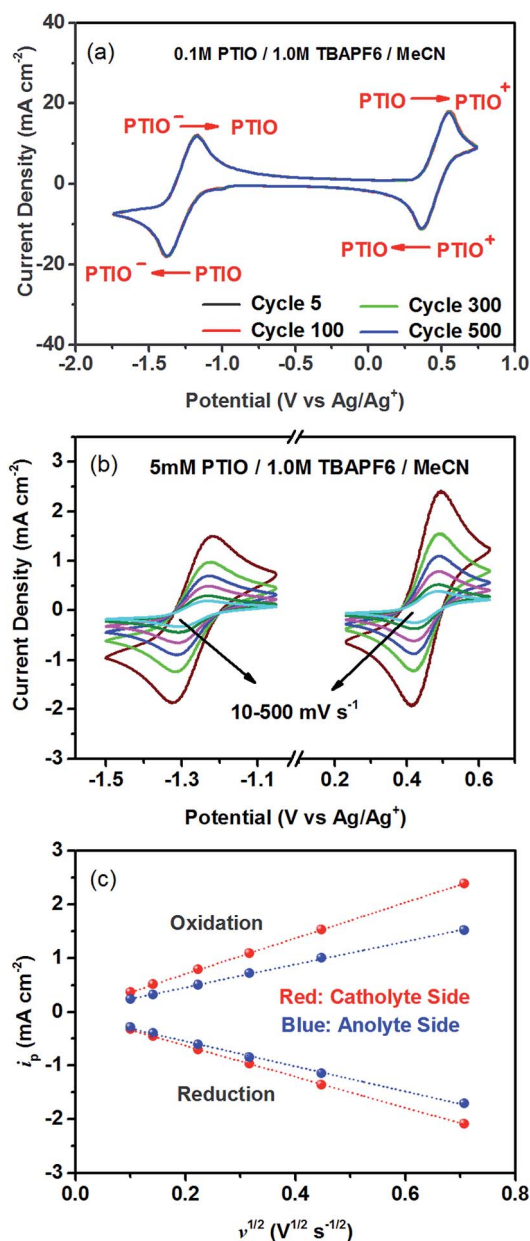
Fig. 1 CV curves of PTIO in a supporting electrolyte of 1.0 M TBAPF 6 /MeCN: (a) 500 cycles of repeated CV scans with 0.1 M PTIO at 100 \text{ mV s}^{-1} ; (b) at different potential sweeping rates ( \nu = 10, 20, 50, 100, 200 and 500 \text{ mV s}^{-1} ) with 5.0 mM PTIO; (c) linear relationship between i_p and \nu^{1/2} obtained from Randles–Sevcik analysis.
