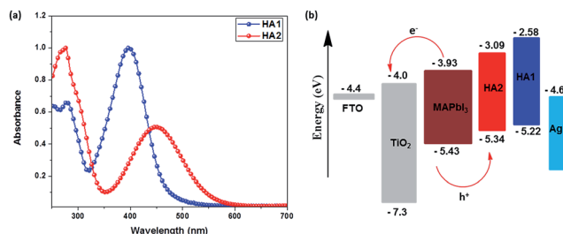
Fig. 2 (a) UV-vis absorption of HA1 and HA2 in \text{CH}_2\text{Cl}_2 solution. (b) Energy level diagram.
