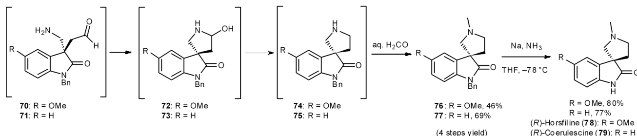
Scheme 7 Three-pot synthesis of (R)-horsifilene and (R)-coerulescine.
