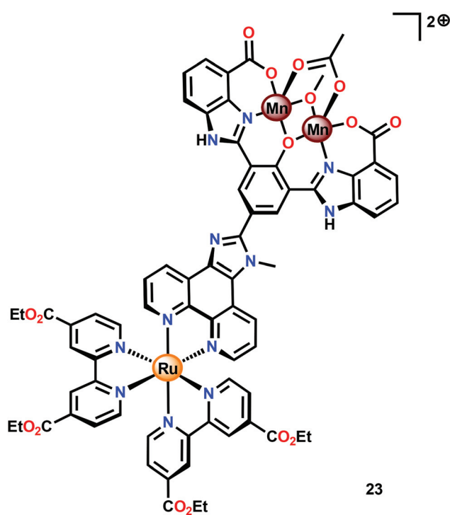
Fig. 11 Structure of Ru–Mn 2 assembly 23 .
