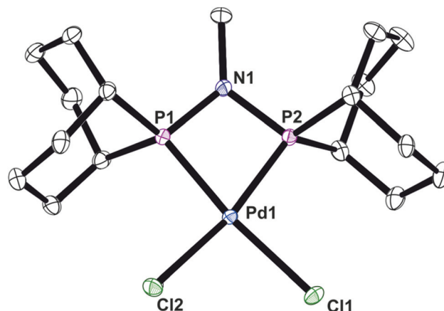
Fig. 6 Crystal structure of complex [\text{PdCl}_2(\text{L}_c)] ( 6 ). All hydrogen atoms have been omitted for clarity. Selected bond lengths (Å) and angles (°); Pd(1)–P(1) 2.2311(4), Pd(1)–P(2) 2.2353(4), Pd(1)–Cl(2) 2.3735(4), Pd(1)–Cl(1) 2.3748(4), P(1)–N(1) 1.6949(14), P(2)–N(1) 1.7016(14), P(1)–Pd(1)–P(2) 70.851(15).
