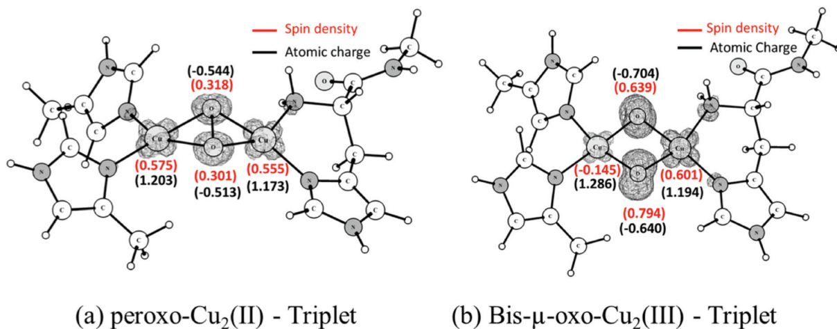
Fig. 4 Calculated Mulliken spin densities and atomic charges for the triplet state of peroxo-Cu(II) 2 and bis( \mu -oxo) \text{Cu(III)}_2 complexes. Spin densities are shown in red and atomic charges in black.
