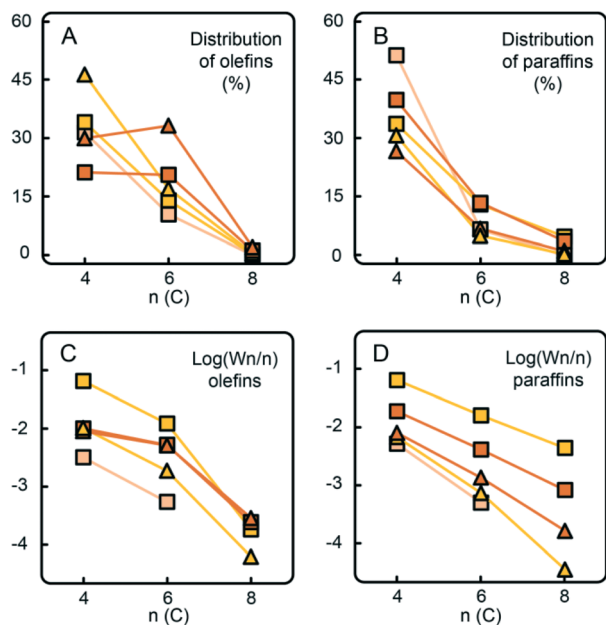
Fig. 11 The increase of Cr loading in the Phillips-type catalyst (from light yellow to orange) increases the selectivity towards C6 products in the experiments with (□) and without (△) hydrogen. A different trend in the distribution of olefinic species (A) compared to paraffinic species (B), also visible in the Schulz-Flory plots (C and D), causes a discrepancy from linearity with increasing Cr loading. A higher amount of Cr, while keeping the Ti loading constant, increases the amount of ethylene trimerisation sites, which produce higher amounts of 1-hexene.
