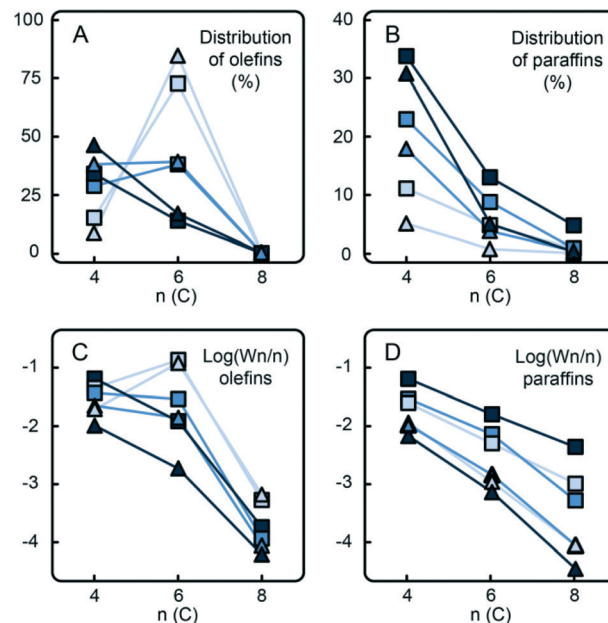
Fig. 10 The increase of Ti loading in the Phillips-type catalyst (from light to dark blue) shifts the selectivity towards C4 at the expense of C6 products in the experiments with ( \square ) and without ( \Delta ) hydrogen. A different trend in the distribution of olefinic species (A) compared to paraffinic species (B) is also clearly visible in the Schulz-Flory plots. While paraffinic species show linear curves independent of the Ti loading (D), olefinic species exhibit a discrepancy from linearity with increasing Ti loading (C), indicating an oligomerisation mechanism, which does not follow SF distribution.
