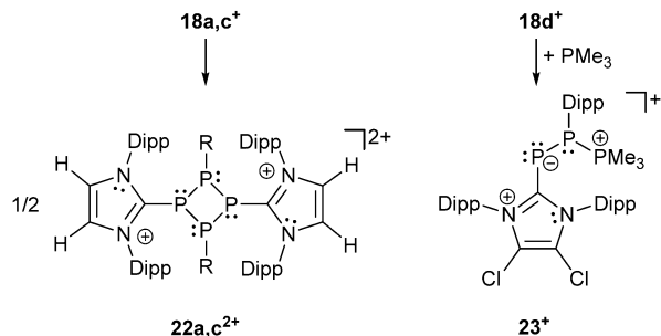
Scheme 8 [2+2] dimerization reaction of diphosphenes 18a,c + (left) and \text{PMe}_3 attacking the more electrophilic P atom of diphosphene 18d + forming \sigma^2\text{-}\sigma^3\text{-}\sigma^4 compound 23 + (right).
