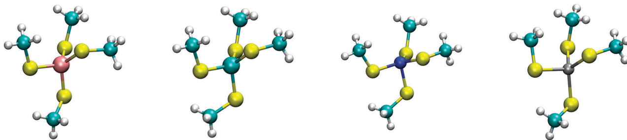
Fig. 1 DFT optimized structures of [(CH_3S)_4M]^{2-} complexes. From left to right, Fe 2+ , Co 2+ , Ni 2+ , and Zn 2+ high spin complexes are shown with multiplicities of 5, 4, 3, and 1, respectively.
