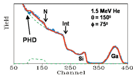
Fig. 6 Non-linearity of the RBS spectrometer. The sample is a 75 \times 10^{15} \text{ Ga cm}^{-2} implant at 75 keV into a 125 nm \text{SiN}_x\text{:H} thin film grown on Si. The detector is placed at a backscattering angle of 150^\circ and the sample normal is at 75^\circ to the beam direction. “Int” labels the \text{SiN}_x/\text{Si} interface as seen in the Si signal. The spectrum (red: calculated assuming linearity) fits the data (blue) perfectly except for the N interface signal (arrowed). “PHD” is the pulse-height defect (see text). Adapted with permission from Fig. 1 of Jeynes et al. , Anal. Chem. , 2012 73 (©2012, American Chemical Society); after Fig. 6 of Jeynes et al. , J. Phys. D: Appl. Phys. , 2003. 3 © IOP Publishing (reproduced with permission, all rights reserved); and redrawn from Nucl. Instrum. Methods Phys. Res., Sect. B , 148, Barradas et al. , RES and ERDA study of ion beam synthesised amorphous gallium nitride, 463–467, (©1999), 94 with permission from Elsevier.
