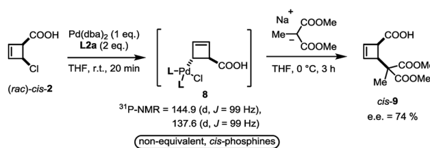
Scheme 4 Formation of four membered ring \eta^1 -allyl complex from cis - 2 .
