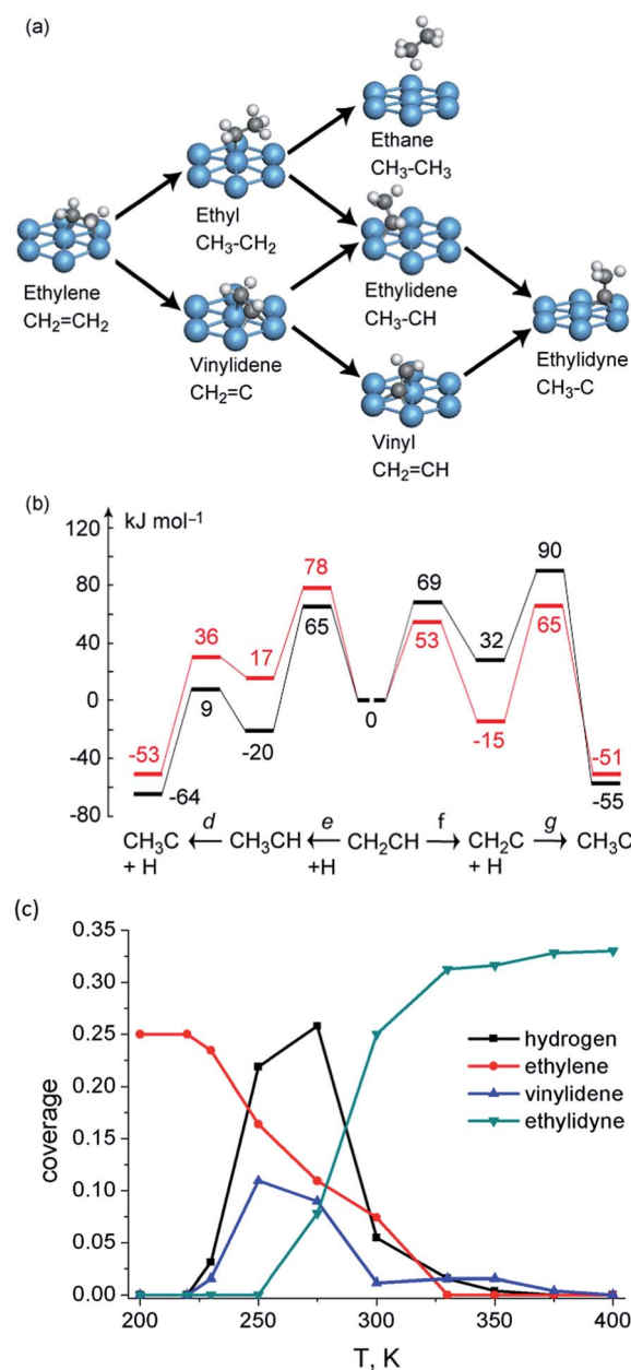
Fig. 5 (a) Reaction network of ethylene transformation over Pt(111); (b) reaction energy profiles ( \text{kJ mol}^{-1} ) of vinyl conversion to ethylidyne over Pt(111) at 1/3 coverage (black) and 1/9 coverage (red). Reprinted with permission from ref. 74. Copyright 2010 American Chemical Society; (c) kMC simulated surface coverage after 1 s reaction over Pt(111). Reprinted with permission from ref. 79. Copyright 2012 Elsevier.
