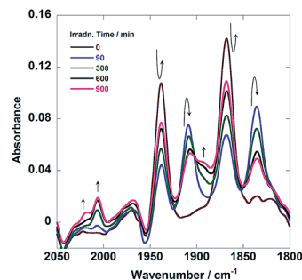
Fig. 7 In situ IR spectra of a DMF–TEOA (5 : 1 v/v) solution containing Ru(CH 2 OCH 2 )Re (1 mM) and BNAH (0.1 M) during photoirradiation at \lambda = 480 nm under a CO 2 atmosphere.
