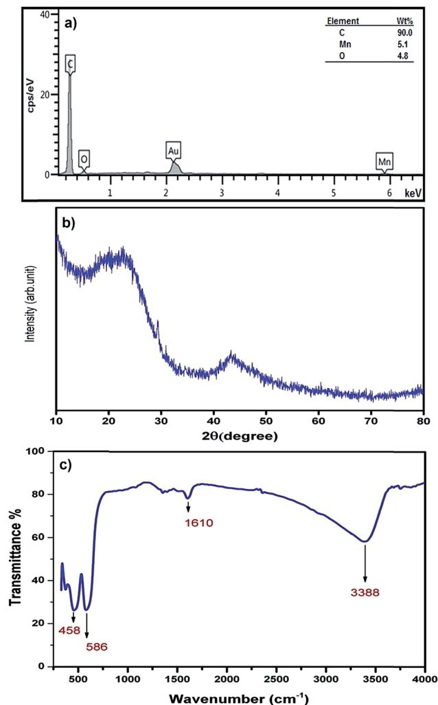
Fig. 5 (a) EDX analysis, (b) XRD pattern and (c) FTIR spectrum of \text{MnO}_2 -NP-AC.
