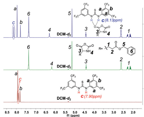
Fig. 2 Expanded ^1\text{H} NMR spectra of TU-S, Glu-NCA and TU-S/Glu-NCA (1 : 1) mixture (500 M, 25 ^\circ\text{C} , \text{CD}_2\text{Cl}_2 , for full spectra see Fig. S1 and S2†).
