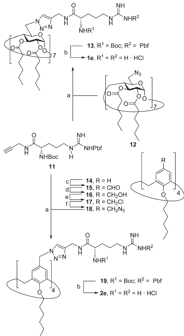
Scheme 3 Synthesis of triazol-linked polyarginine \beta CD and CA 4 "clicked" clusters 1e and 2e . Reagents and conditions: (a) CuI·P(OEt) 3 , DIPEA, acetone, reflux, 48 h, 99% (for 13 ) or 24 h, 71% (for 19 ); (b) (i) 95 : 2.5 : 2.5 TFA–TIS–H 2 O, rt, 1 h; (ii) 0.1 M HCl, quantitative; (c) (i) hexamethylenetetramine, TFA, reflux, 2 d; (ii) HCl, 3 h, 96%; (d) NaBH 4 , EtOH, 0 °C → rt, 18 h, 86%; (e) SOCl 2 , DCM, 4 h, rt, 95%; (f) NaN 3 , DMF, 16 h, 40 °C, 95%.
