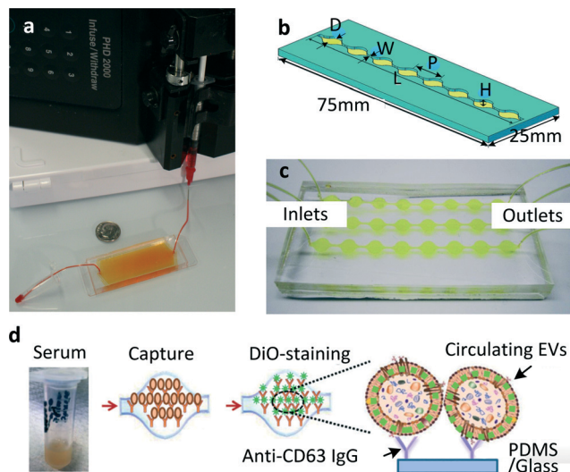
Fig. 1 (a) The first chip realised for microfluidic exosome isolation featured a 19\text{ mm} \times 20\text{ mm} \times 4.5\text{ cm} chamber with herringbone groves 10\text{ }\mu\text{m} deep to enhance contact between microparticles and chip surface. The device is pictured here is filled with supernatant fluid and attached to a syringe pump. Reproduced from ref. 23 with the permission of the Royal Society of Chemistry. (b) A modified version of the same scheme: single channel Exochip, the device has the same dimensions of a standard glass-side ( W = 0.75\text{ mm} , L = 73\text{ mm} , P = 9\text{ mm} , H = 100\text{ }\mu\text{m} ). Up to 12 channels could fit within the dimensions of a microtiter-plate. (c) Experimental setup using a 3 channels Exochip (d) Exochip working scheme: exosomes counting is made possible through a simple 3 steps procedure involving: (i) blood serum infusion within the chip (pre-coated with exosome-specific capture antibodies, anti-CD63), (ii) staining with specifically functionalised (Di-O) fluorescent dye, (iii) on chip analysis through conventional counting methods. Reproduced from ref. 22 with the permission of the Royal Society of Chemistry.
