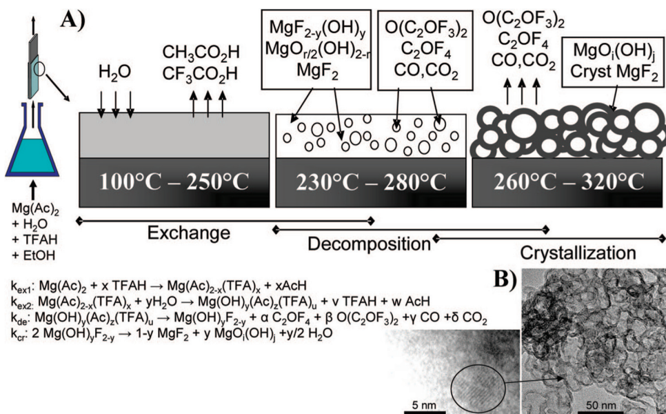
Fig. 1 (A) Scheme representing the deposition of porous MgF_2 films on Si substrates by the TFA route; (B) TEM images showing the vesicle-like structures of the film prepared at 10\text{ }^{\circ}\text{C min}^{-1} under a dry atmosphere. Reprinted with permission from ref. 6a. © 2015 American Chemical Society.
