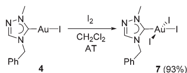
Scheme 5 Synthesis of \text{Au(III)} triiodido complex 7 .
