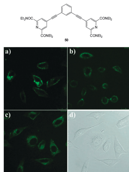
Fig. 45 Top: structure of dialkynylbenzene probe 50 . Bottom: in vitro cytoplasmic staining microscopy with 50 ( \lambda_{\text{ex}} = 900 \text{ nm} , \lambda_{\text{em}} = 450\text{--}750 \text{ nm} ) in A549 cells after (a) 1 h, (b) 6 h, and (c) 12 h. (d) Bright-field image of panel (c). Image reproduced with permission. 198
